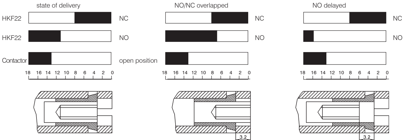
Stand position of regulation screw
